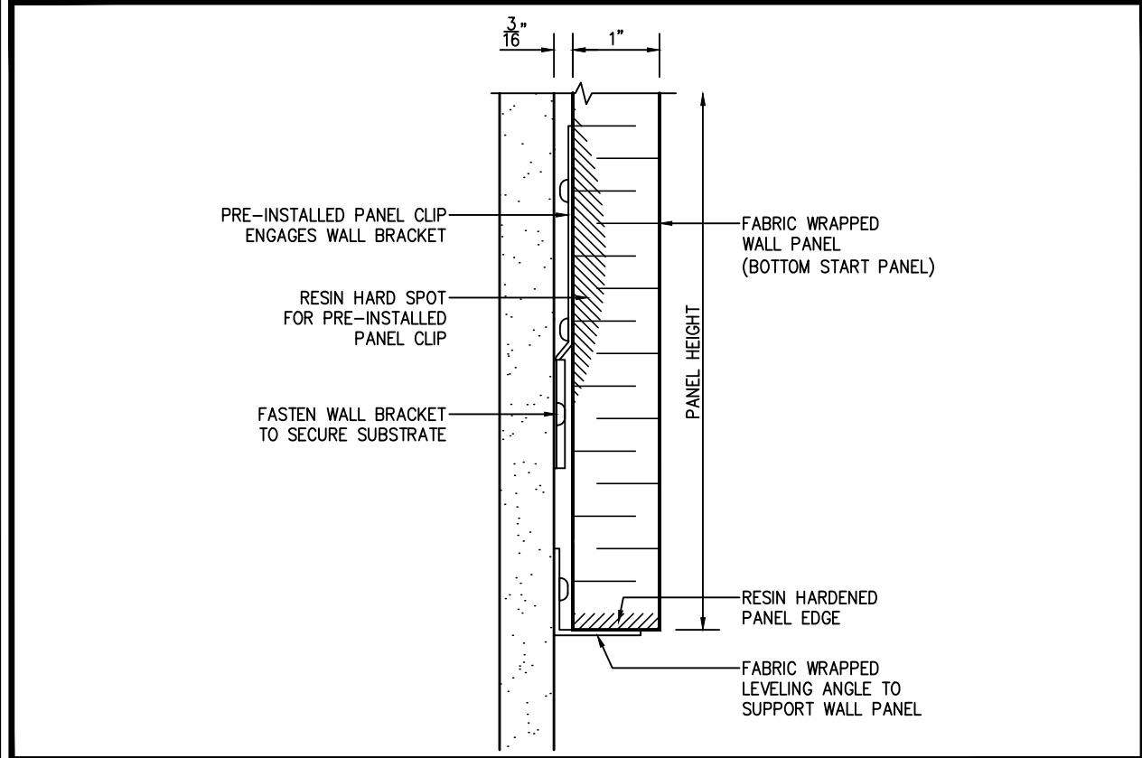
2 ELEVATION SECTION - BASE OF PANEL D1 SCALE 6"=1'-0"
