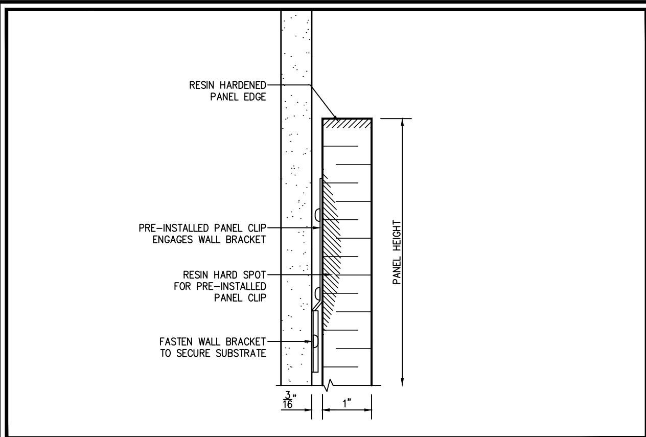
1 ELEVATION SECTION - TOP OF PANEL D1 SCALE 6"=1'-0"
