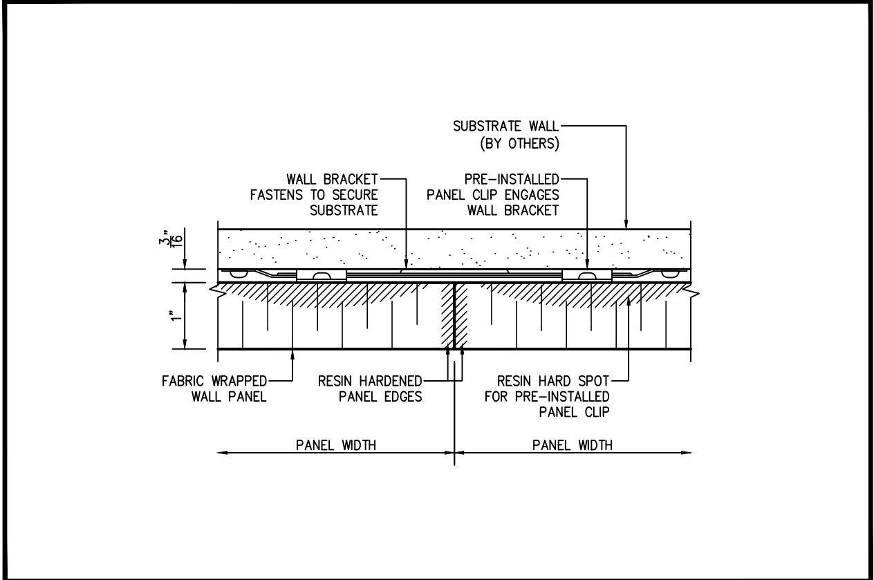
4 PLAN SECTION - VERTICAL JOINT D1 SCALE 6"=1'-0"
