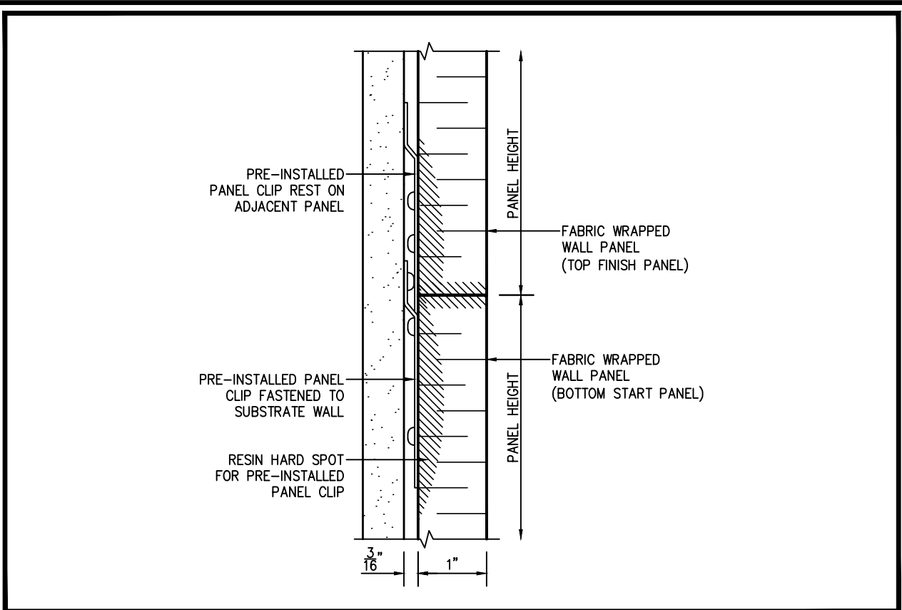
3 ELEVATION SECTION - HORIZONTAL JOINT D1 SCALE 6"=1'-0"
