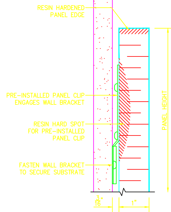
1 ELEVATION SECTION - TOP OF PANEL D1 SCALE 6"=1'-0"
