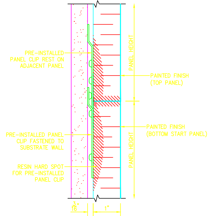
3 ELEVATION SECTION - HORIZONTAL JOINT D1 SCALE 6"=1'-0"
