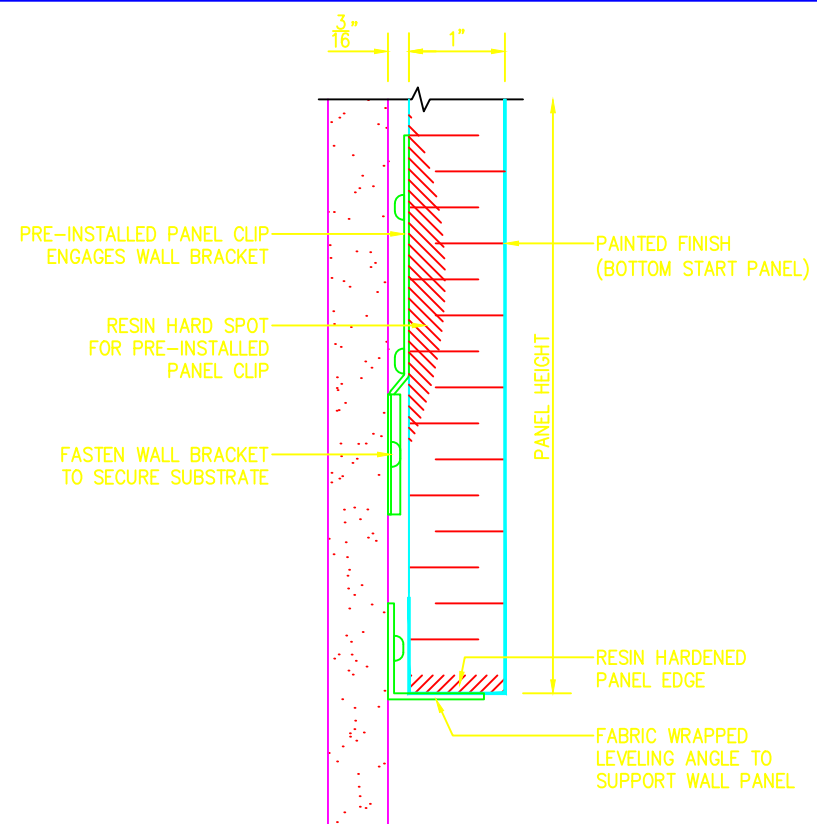
2 ELEVATION SECTION - BASE OF PANEL D1 SCALE 6"=1'-0"
