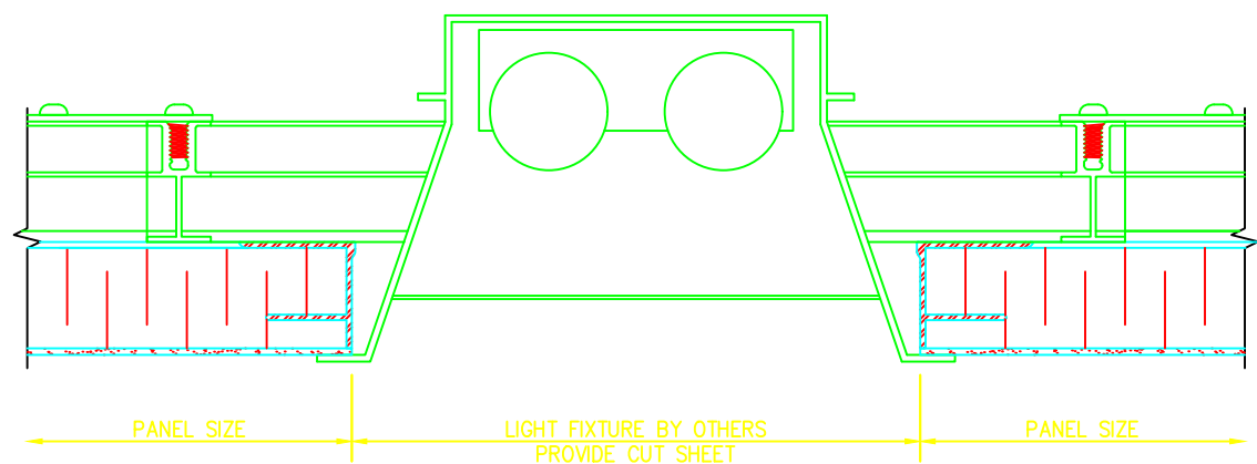
3 LINEAR LIGHT FIXTURE WITH FLANGE D2 SCALE 6"=1'-0"
