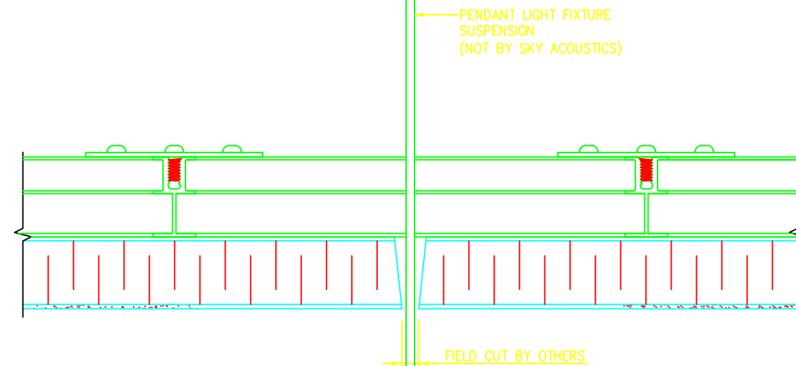
4 PENDANT LIGHT DETAIL (BOXED OUT GRID) D2 SCALE 6"=1'-0"
