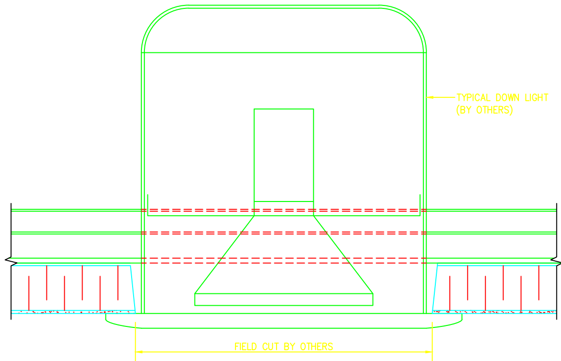
1 FIELD CUT DETAIL FOR FIXTURES D2 SCALE 6"=1'-0"
