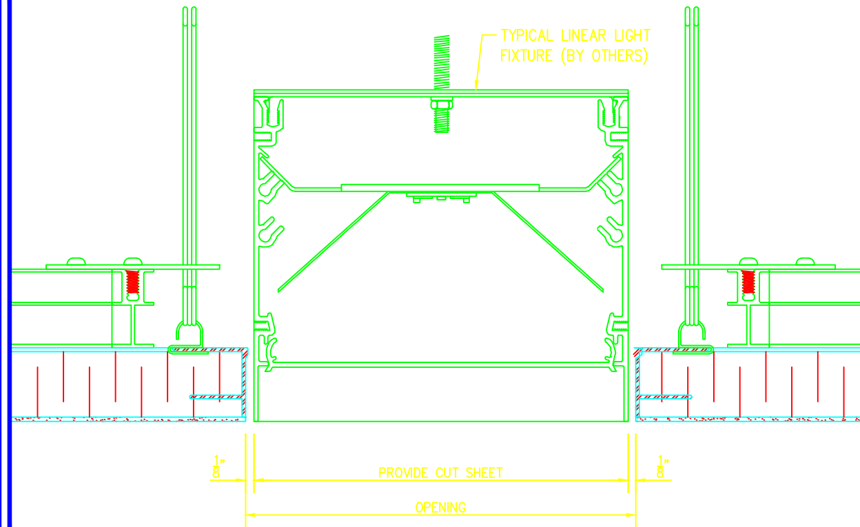
2 LINEAR LIGHT FIXTURE DETAIL D2 SCALE 6"=1'-0"
