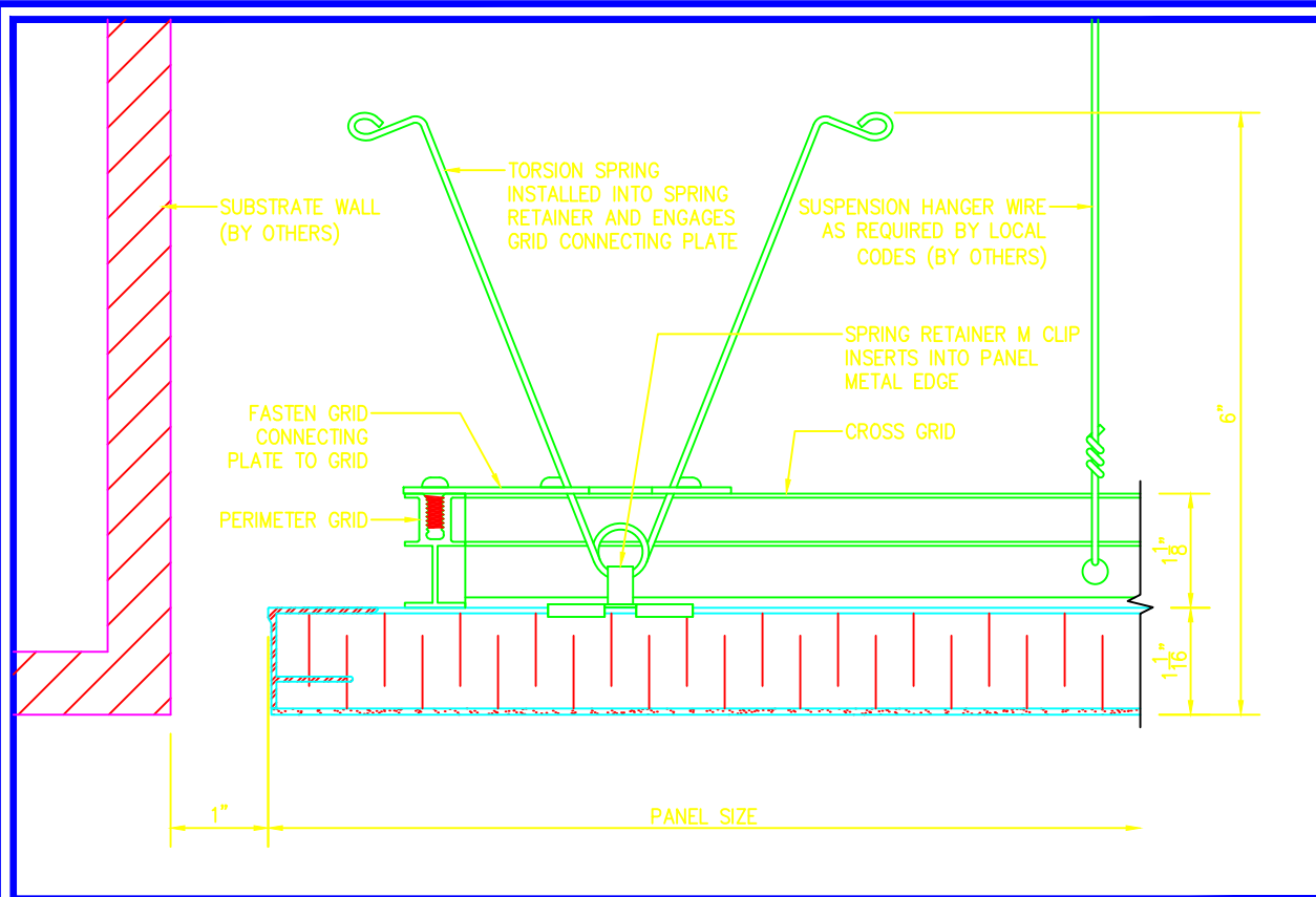
1 PERIMETER PANEL DETAIL D1 SCALE 6"=1'-0"
