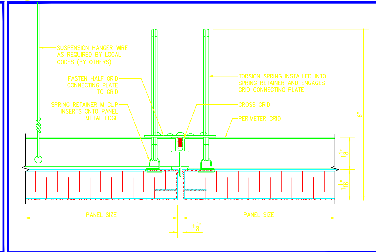
4 DEFINED JOINT DETAIL D1 SCALE 6"=1'-0"
