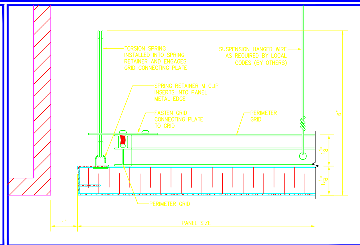
2 PERIMETER PANEL DETAIL D1 SCALE 6"=1'-0"
