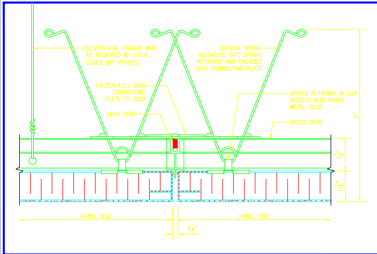
3 DEFINED JOINT DETAIL D1 SCALE 6"=1'-0"
